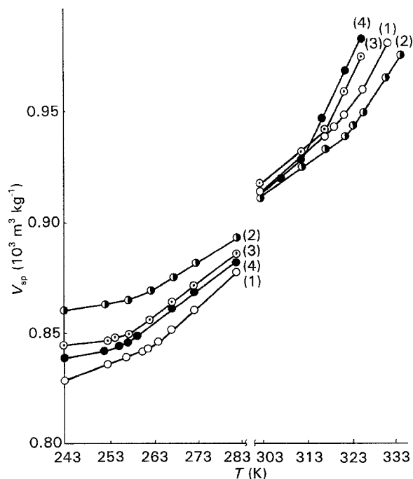
Figure 2 Temperature dependence of specific volume for gradient IPN sections sliced off perpendicular to the BMA + TrEGDMA copolymer concentration gradient. Sections are numbered from surface to core of the gradient system [10].
