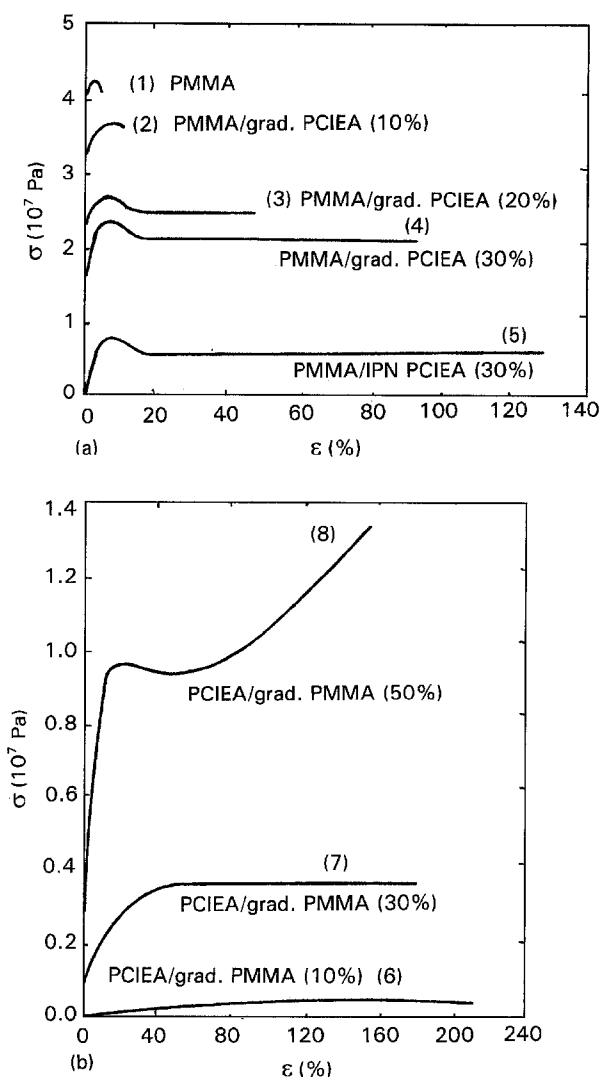
Figure 9 Stress-strain curves for: (a) PMMA (1); gradient IPNs (2-4) and ordinary IPN (5) with PMMA matrix, containing (2) 10, (3) 20, and (4, 5) 30 mass% PCIEA; (b) gradient IPNs with PCIEA matrix, containing (6) 10, (7) 30, and (8) 50 mass% PMMA. Strain rate = 0.042 \text{ s}^{-1} ; temperature = 60^\circ \text{C} [9].
