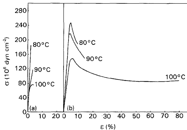
Figure 6 Stress-strain curves for (a) ordinary and (b) gradient IPNs at various temperatures. Total methyl acrylate content in PMMA is 20% in both samples [1].
